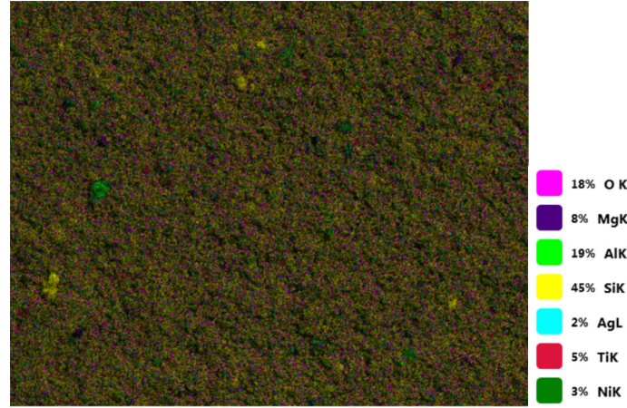
Figure 7. SEM mapping result of Ag-Ni-TiO 2 /Cordierite catalyst
