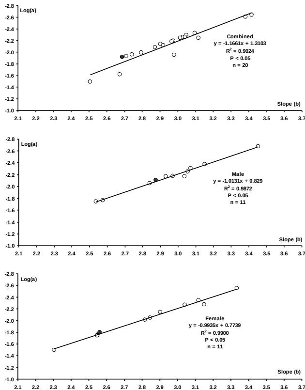
Figure 2. The test plot of \log(a) against b for different WLRs of the Anchovy ( Engraulis encrasicolus ). Black dot = present study parameter. White dot = estimated parameters of different studies conducted from 1985-1986 to 2013-2014 fishing seasons in the Black Sea (see Table 2).
