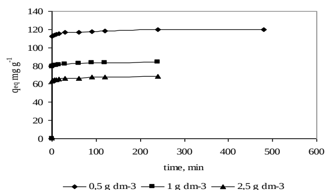
Figure 3. Influence of adsorbent dosage in adsorption yield and equilibrium uptake ( C_0 = 100 mg L -1 , pH= 4.0, T= 60 °C, X: 0.5 g L -1 , agitation rate= 150 rpm).
