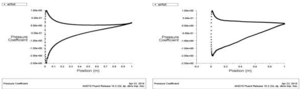
Figure 22. Pressure coefficient of NACA0012 and NACA4412 at 8° angle of attack
