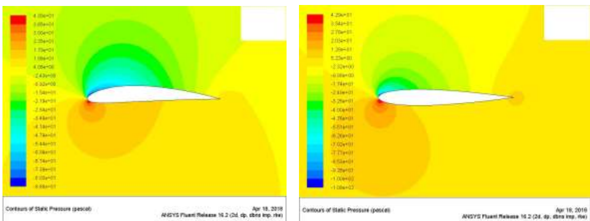
Figure 15. Pressure contours of NACA0012 and NACA4412 at 7° of angle of attack
