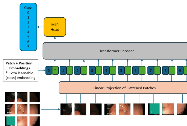
Figure 3. ViTs architecture for endoscopic image classification
