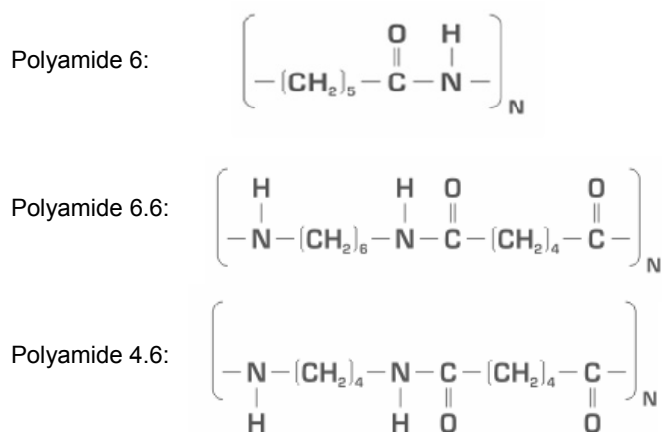
Fig.2. The chemical structures of PA6, PA 6.6 and PA 4.6
