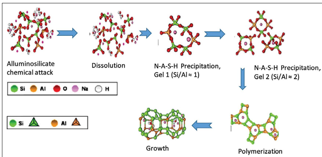
Figure 1. Geopolymerization process [82, 81].
