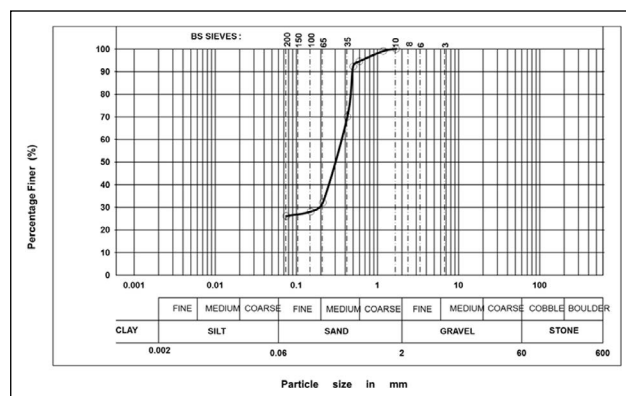
Figure 2. Particle size and Texture of Sharp Sand.
