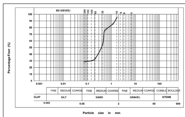
Figure 1. Particle Size and Texture of Iron Tailings.
