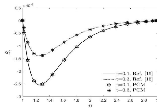
(b) Radial stress distribution
