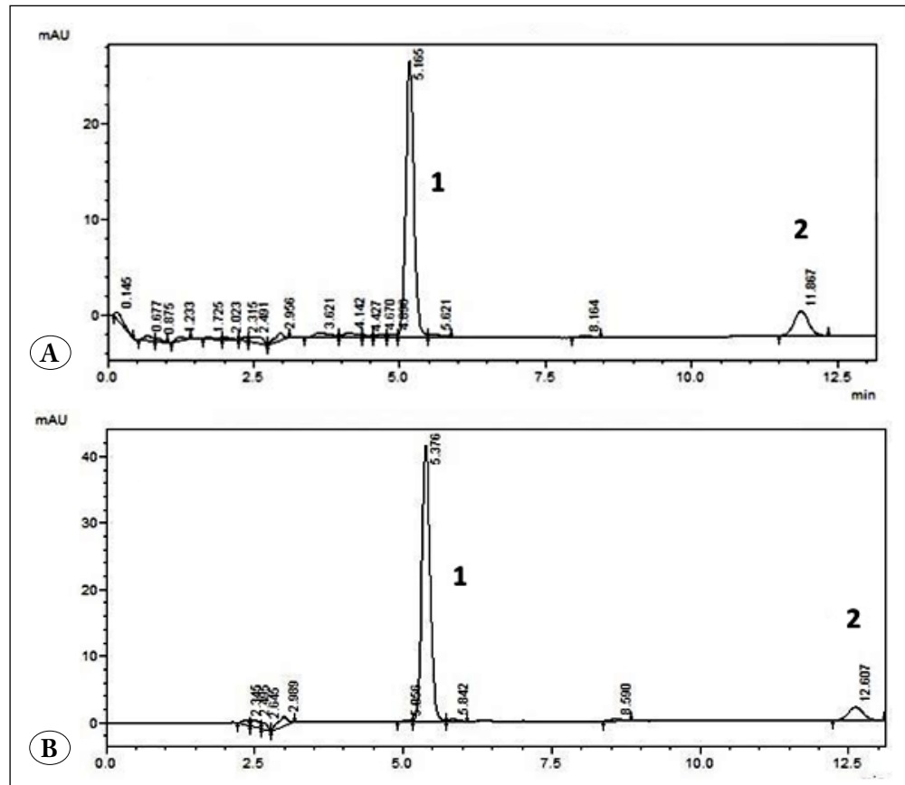
Figure 4. (A) Chromatograms of pravastatin and rosuvastatin (IS) in pharmaceutical dosage form. 1) Pravastatin (4 \mu\text{g/mL} ), 2) Rosuvastatin (IS) (1 \mu\text{g/mL} ), (B) Pharmaceutical dosage form spiked with each drug at 1) Pravastatin (8 \mu\text{g/mL} ), 2) Rosuvastatin (IS) (1 \mu\text{g/mL} ).
