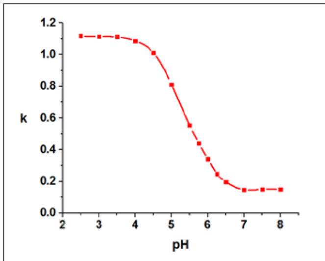
Figure 2. Values of retention factor values vs. pH of the mobile phase for pravastatin on the XTerra C18 column at 25°C using the acetonitrile–water (40:60, v/v) binary mixture. The theoretical results are shown as continuous lines and the plotted points are experimental results.
