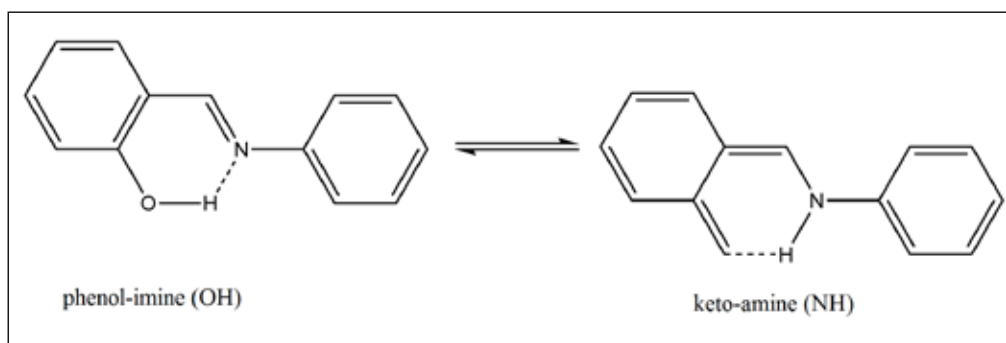
Figure 1. Enol-imine (OH) and keto-amine (NH) forms of o -hydroxy Schiff bases.
