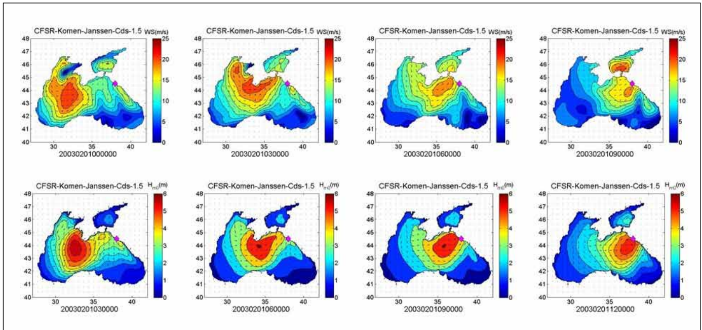
Figure 8. Spatial and temporal development of simulated H_{m0} fields and CFSR wind speed fields and wind and wave direction vectors from the best setting SWAN model simulations forced with the CFSR winds. Pink diamonds in the figures represent the Gelendzhik location.
