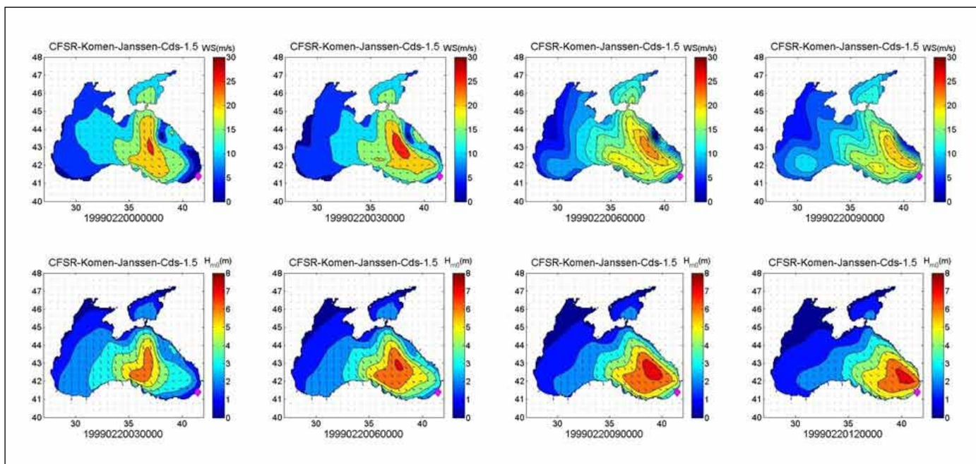
Figure 6. Spatial and temporal development of simulated H_{m0} fields and CFSR wind speed fields and wind and wave direction vectors from the best setting SWAN model simulations forced with the CFSR winds. Pink diamonds in the figures represent the Hopa location.
