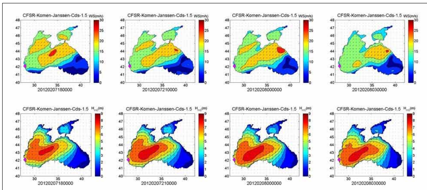
Figure 10. Spatial and temporal development of simulated H_{m0} fields and CFSR wind speed fields and wind and wave direction vectors from the best setting SWAN model simulations forced with the CFSR winds. Pink diamonds in the figures represent the Ahtopol location.
