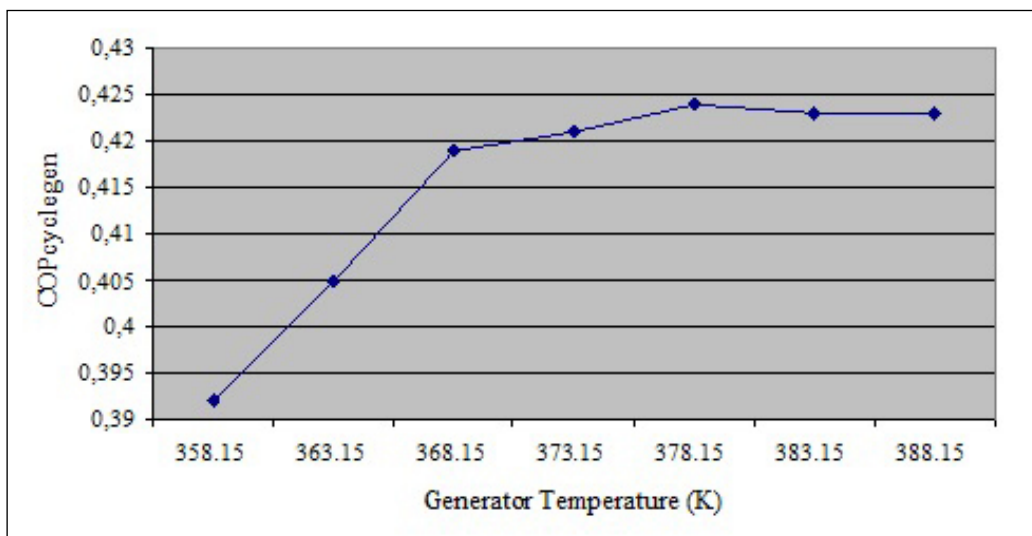
Figure 3. Variation of COP_{cyclegen} with Generator Temperature (K) of the novel cycle.
