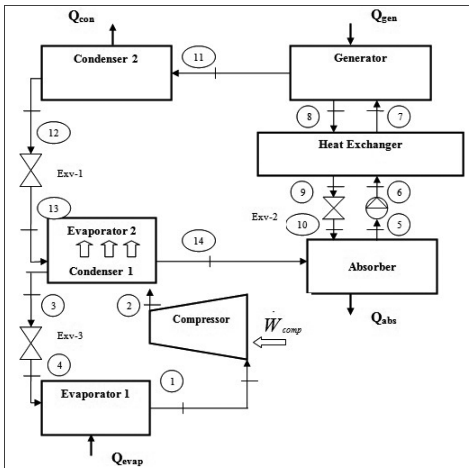
Figure 1. Schematic illustration of the single effect vapour compression-absorption cascade refrigeration cycle.
