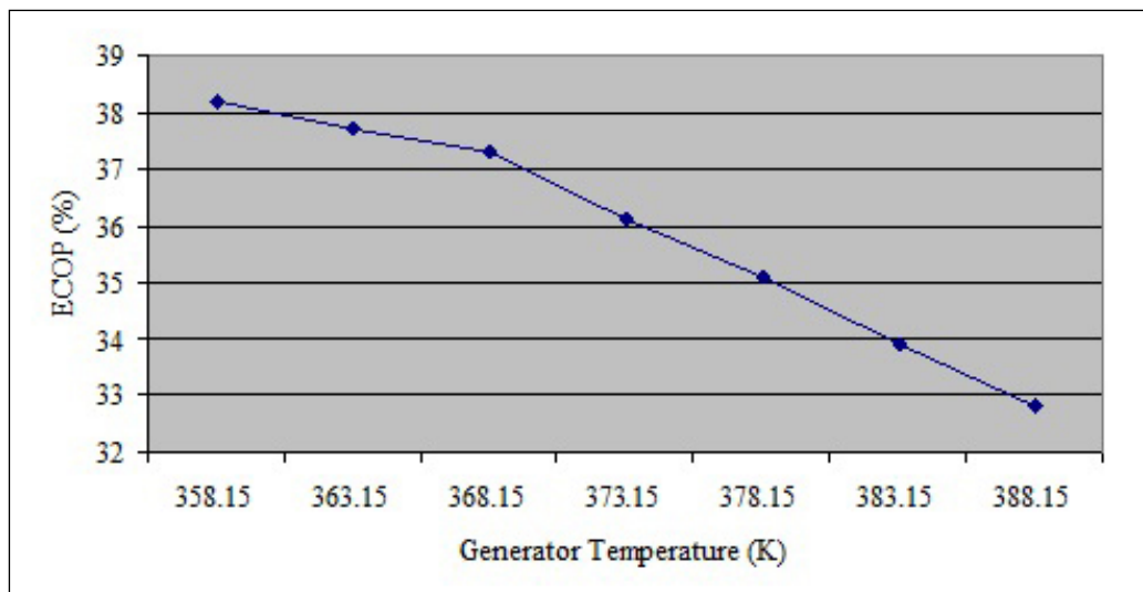
Figure 4. Variation of ECOP with Generator Temperature (K) of the novel cycle.
