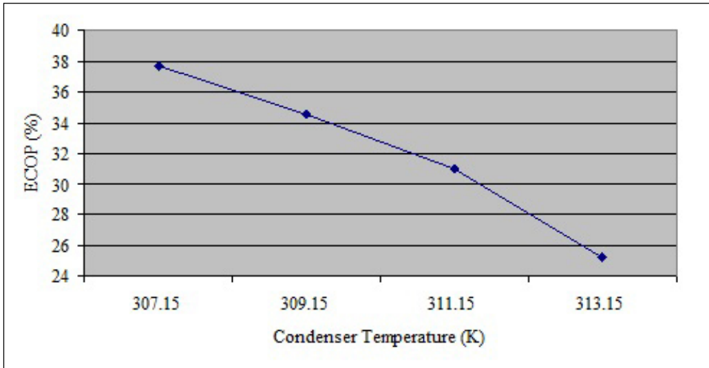
Figure 6. Variation of ECOP with Condenser Temperature (K) of the novel cycle.
