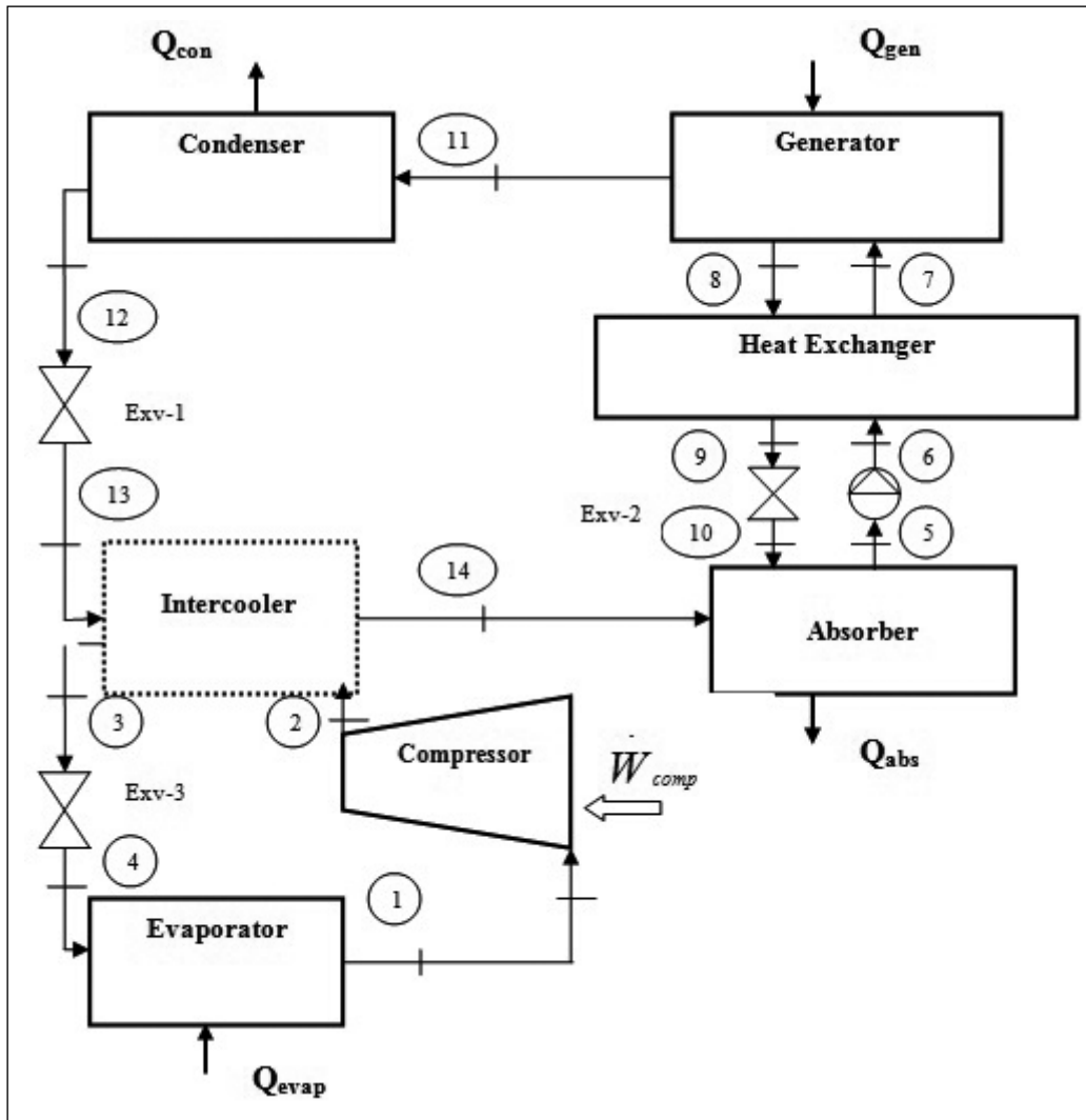
Figure 2. The schematic illustration of the novel cycle.
