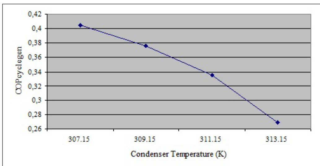
Figure 5. Variation of COP_{cyclegen} with Condenser Temperature (K) of the novel cycle.
