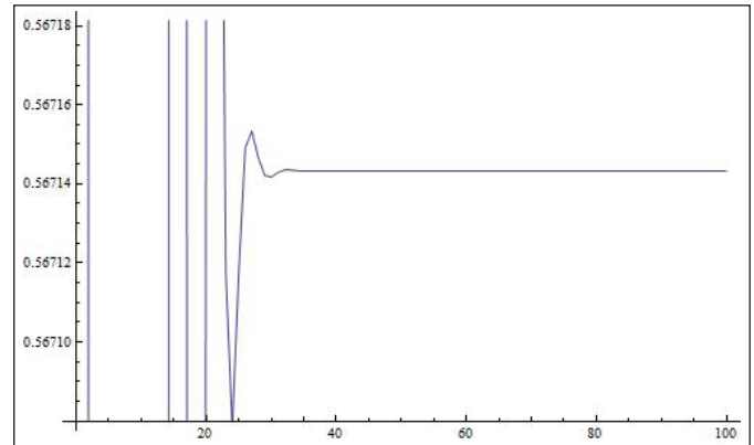
Figure 1. The positive solutions of Eq.(1.4) with k = 1 .
