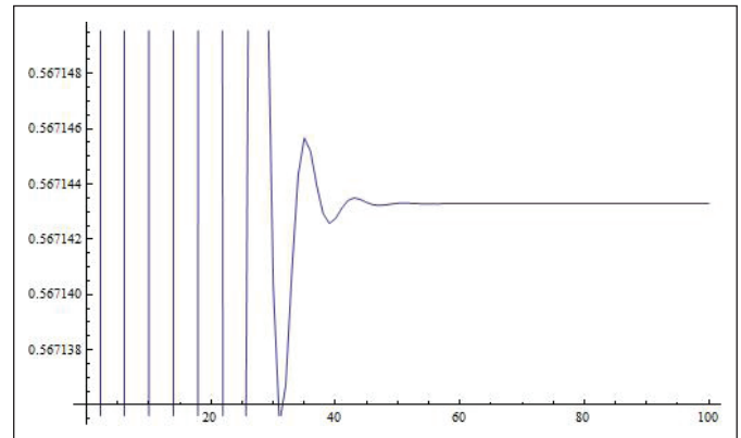
Figure 2. The positive solutions of Eq. (1.4) with k = 2 .
