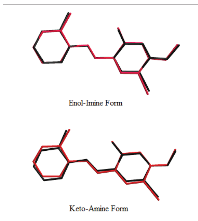
Figure 3. Superimposition of the X-ray structure (red) and calculated structure (black) of the title molecule for enol-keto tautomerism.
