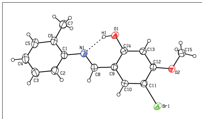
Figure 2. Ortep 3 diagram for the title compound, with the atom numbering scheme. Dashed lines are show the O1-H1...N1 intra molecular hydrogen bonds.
