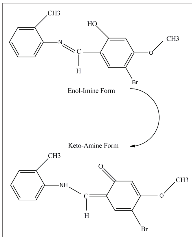
Figure 1. Enol-imine and keto-amine tautomeric forms of title compound.
